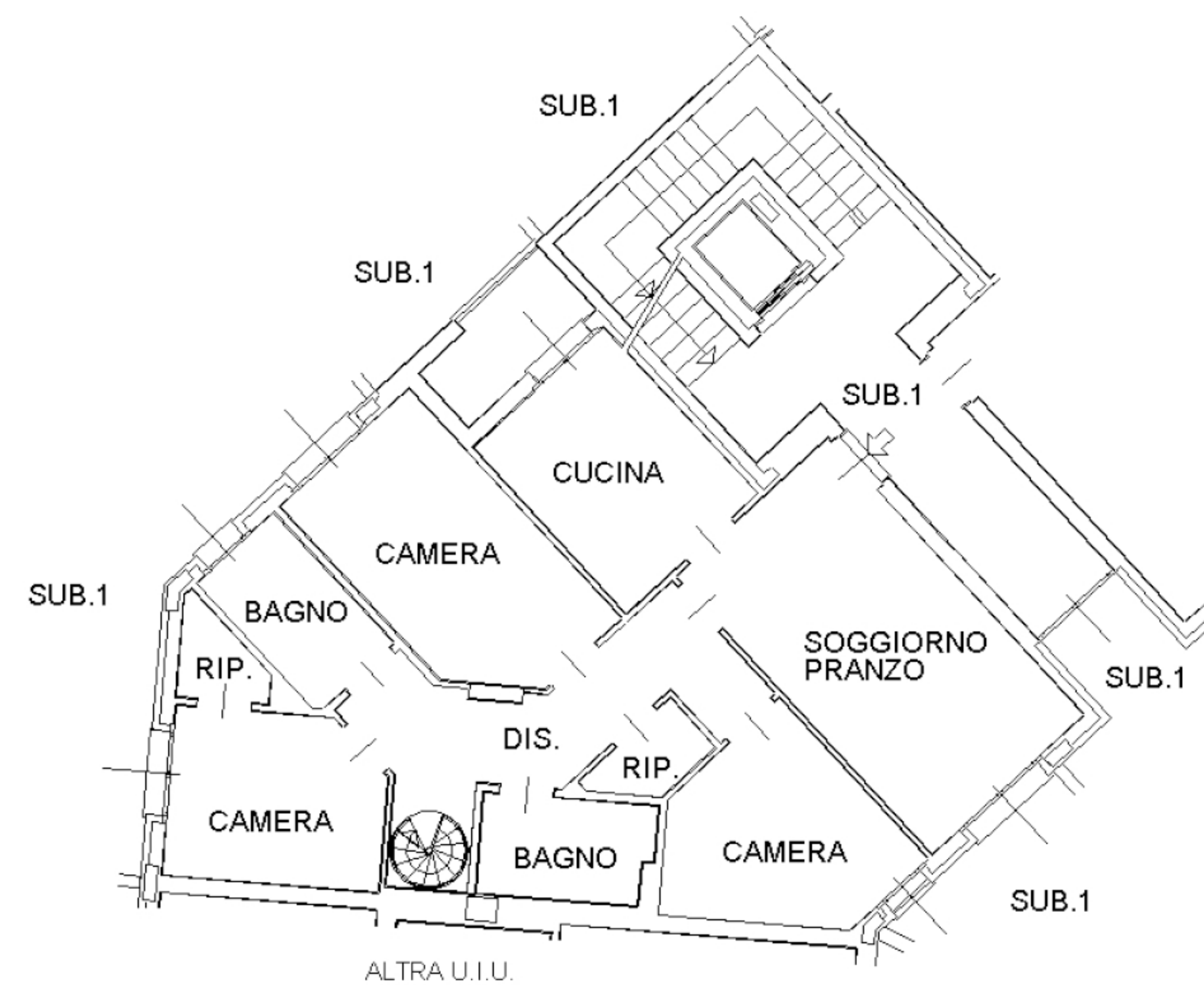
PIANO TERRA - H=2.70
